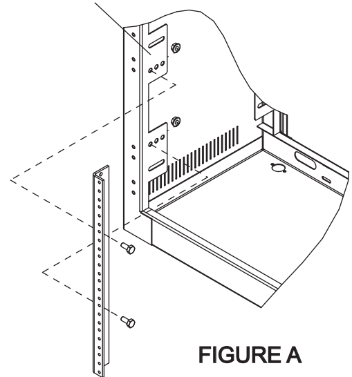
FIXED RACKRAIL BRACKET
