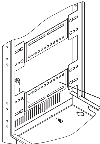
ADJUSTABLE RACKRAIL BRACKET EXTENDER
